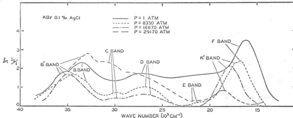
FIG. 7. Typical spectra vs wave number: KBr—0.1% AgCl.
